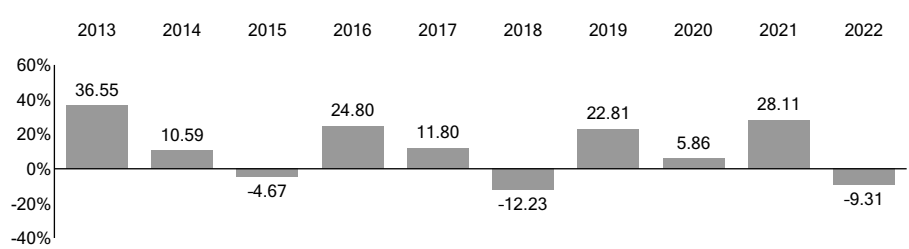
Annual Total Returns — Vanguard Small-Cap Value Index Fund Institutional Shares
